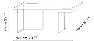
C05D1103.+C07D1107.+C07D1108.
